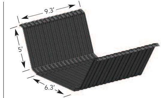
CAD rendering of typical MegaDitch 115° one base and one arm configuration. Each Sidewall Panel section is approximately 5'x9.3'. Each Base Panel section is approximately 6.3'x9.3'
