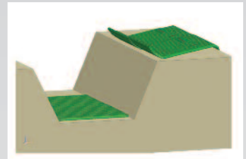
Overlapping base sections placed over the existing channel floor to the desired length and width.
